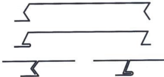
Fig. 7. Complementary interlocking planks, at the top - fitted out with chevron joint, in the middle – fitted out with clip joint, at the bottom – examples of the locked chevron and clip joints.
